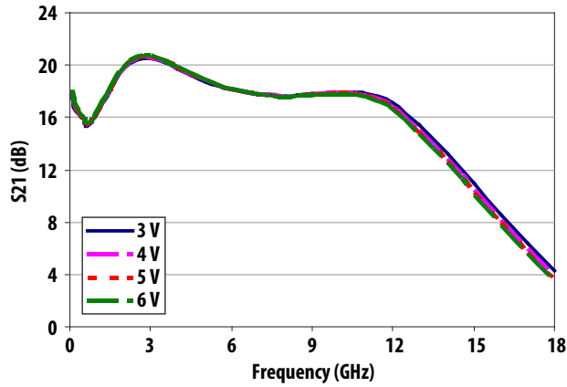
Figure 1. Small Signal Gain over Vdd
